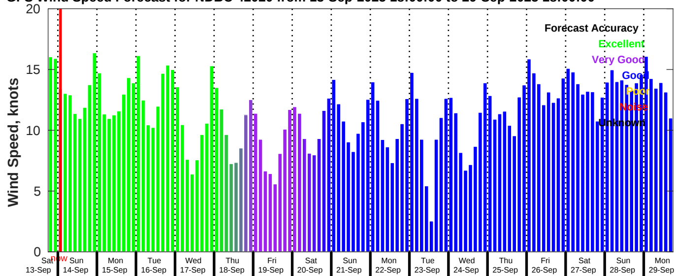
GFS Wind Speed Forecast for NDBC 42020 from 13-Sep-2025 18:00:00 to 29-Sep-2025 18:00:00
