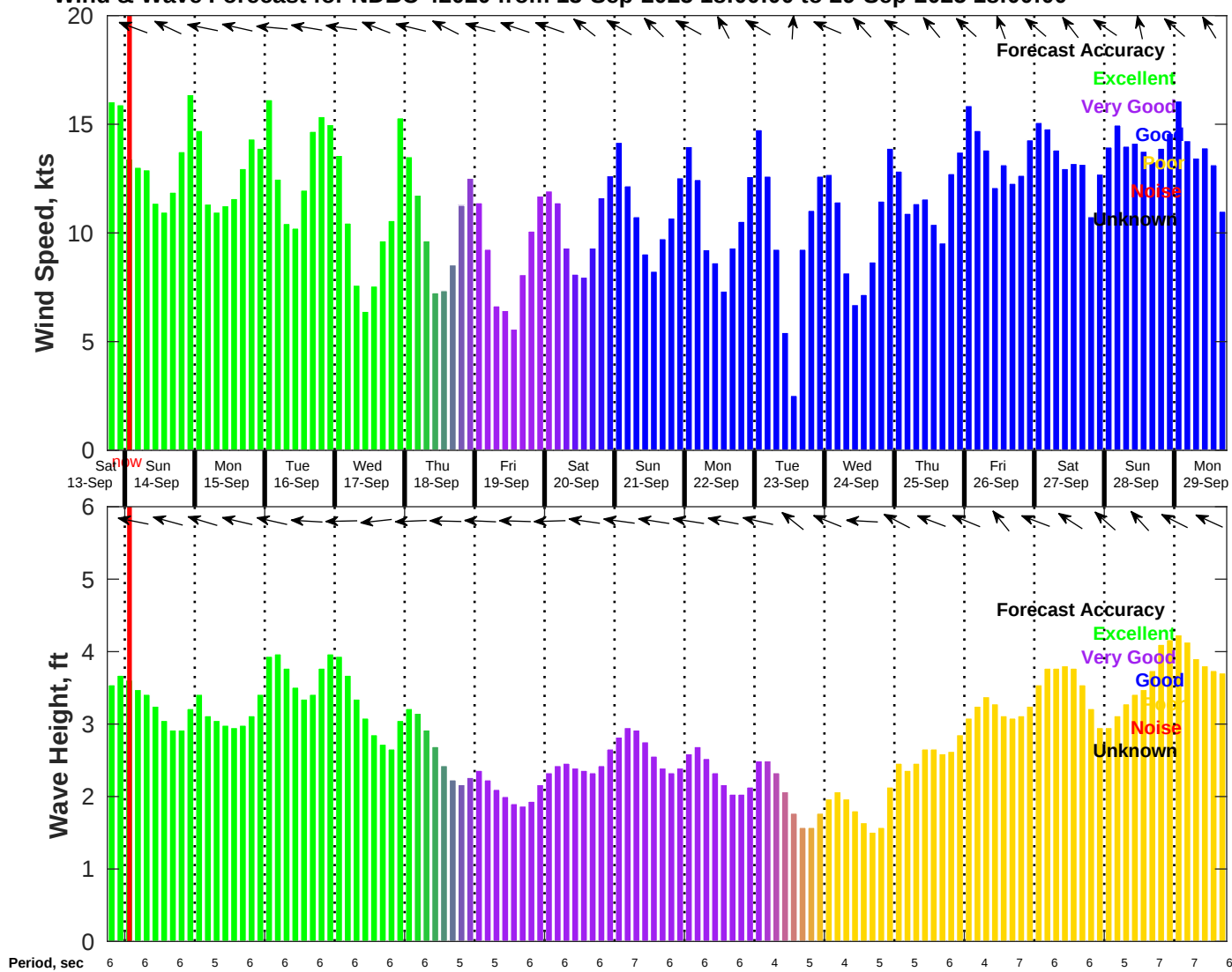
Wind & Wave Forecast for NDBC 42020 from 13-Sep-2025 18:00:00 to 29-Sep-2025 18:00:00
