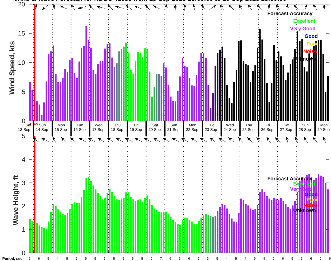
Wind & Wave Forecast for NDBC 42035 from 13-Sep-2025 18:00:00 to 29-Sep-2025 18:00:00
