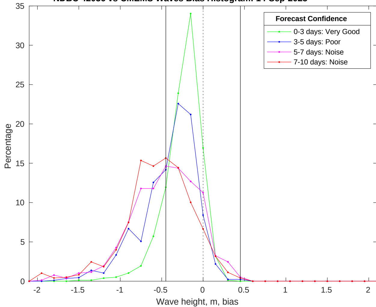
NDBC 42036 vs CMEMS Waves Bias Histogram: 14-Sep-2025
