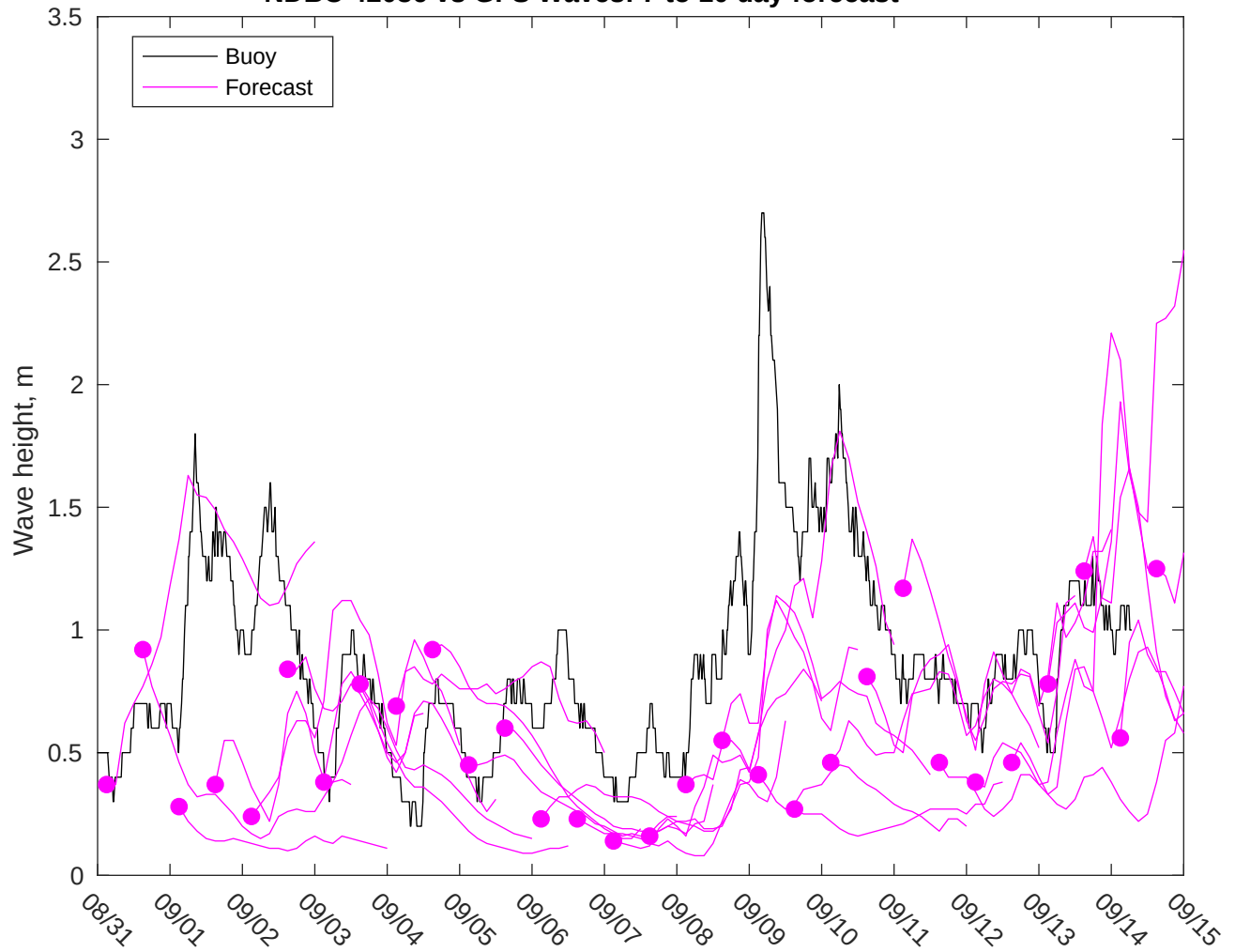
NDBC 42036 vs GFS Waves: 7 to 10 day forecast
