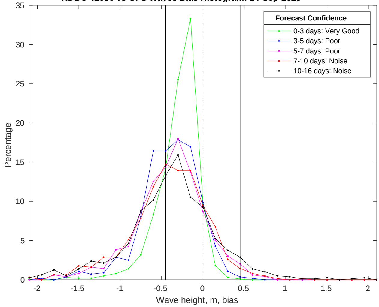
NDBC 42036 vs GFS Waves Bias Histogram: 14-Sep-2025
