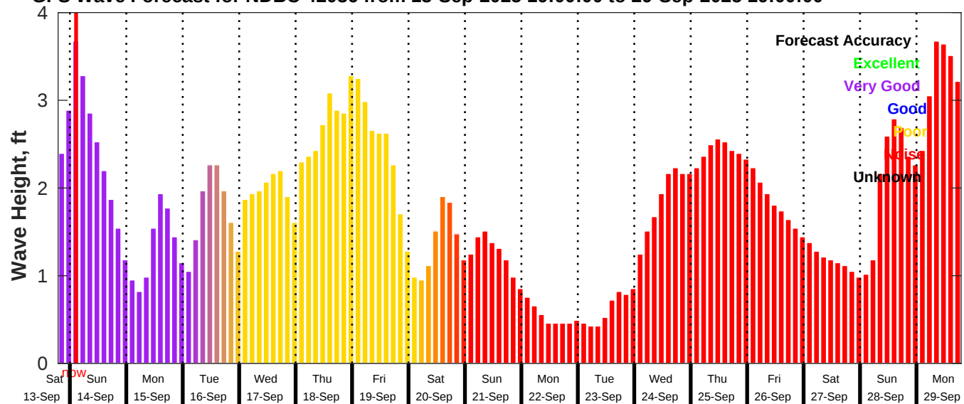
GFS Wave Forecast for NDBC 42036 from 13-Sep-2025 19:00:00 to 29-Sep-2025 19:00:00
