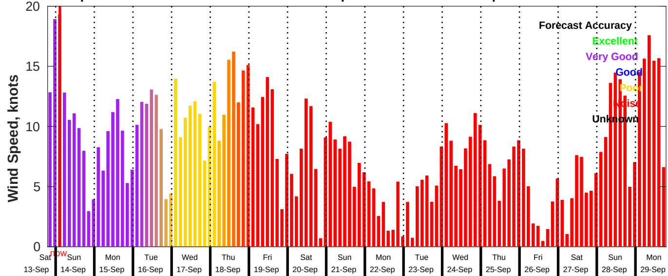
GFS Wind Speed Forecast for NDBC 42036 from 13-Sep-2025 19:00:00 to 29-Sep-2025 19:00:00
