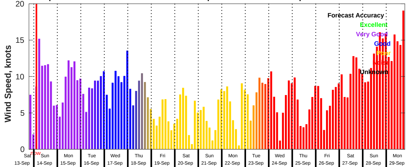
GFS Wind Speed Forecast for NDBC 42040 from 13-Sep-2025 19:00:00 to 29-Sep-2025 19:00:00
