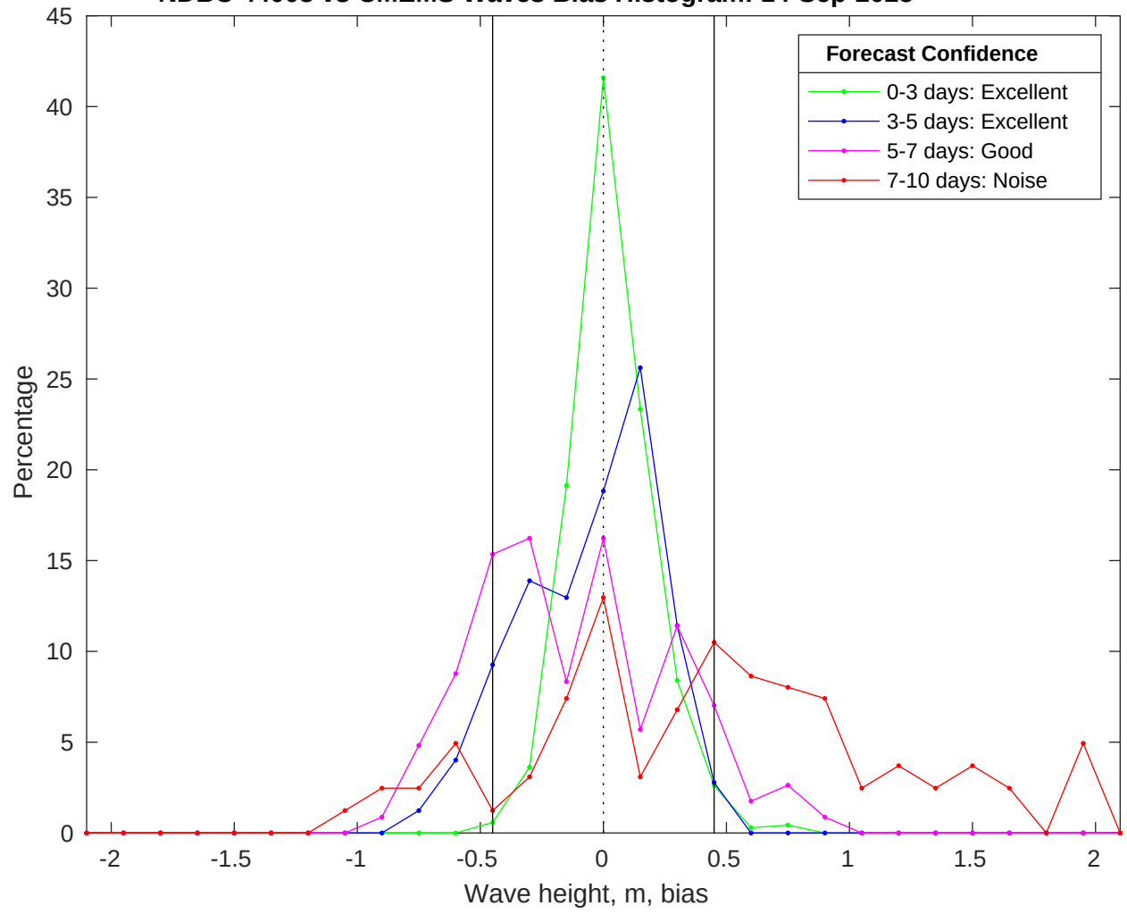
NDBC 44008 vs CMEMS Waves Bias Histogram: 14-Sep-2025
