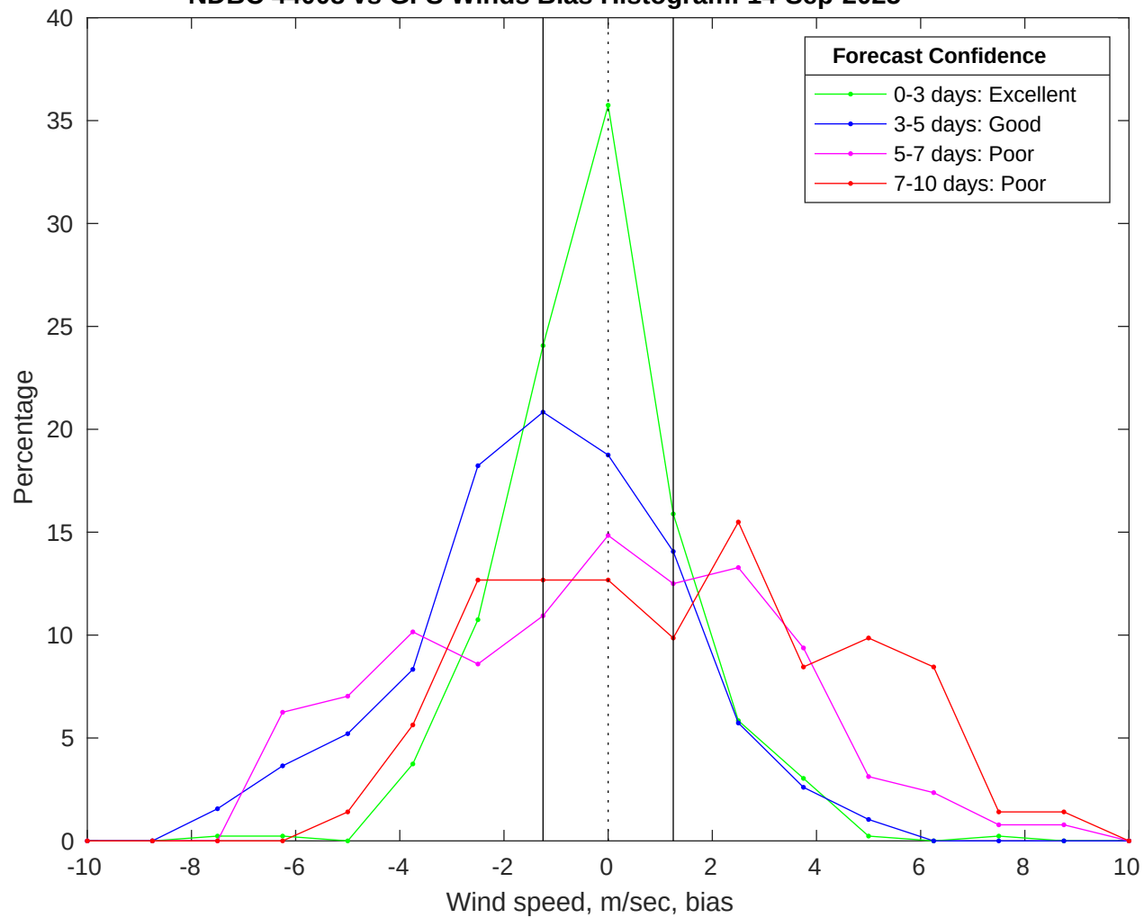
NDBC 44008 vs GFS Winds Bias Histogram: 14-Sep-2025
