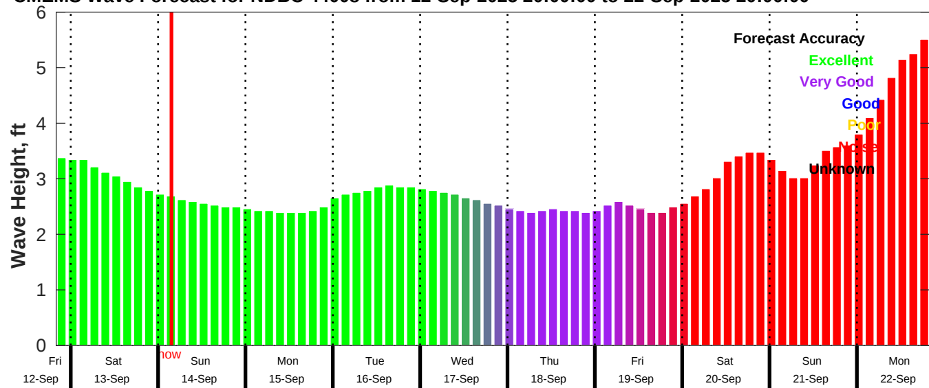
CMEMS Wave Forecast for NDBC 44008 from 12-Sep-2025 20:00:00 to 22-Sep-2025 20:00:00
