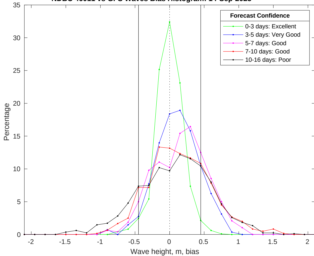
NDBC 46011 vs GFS Waves Bias Histogram: 14-Sep-2025
