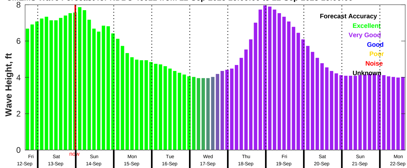
CMEMS Wave Forecast for NDBC 46011 from 12-Sep-2025 16:00:00 to 22-Sep-2025 16:00:00
