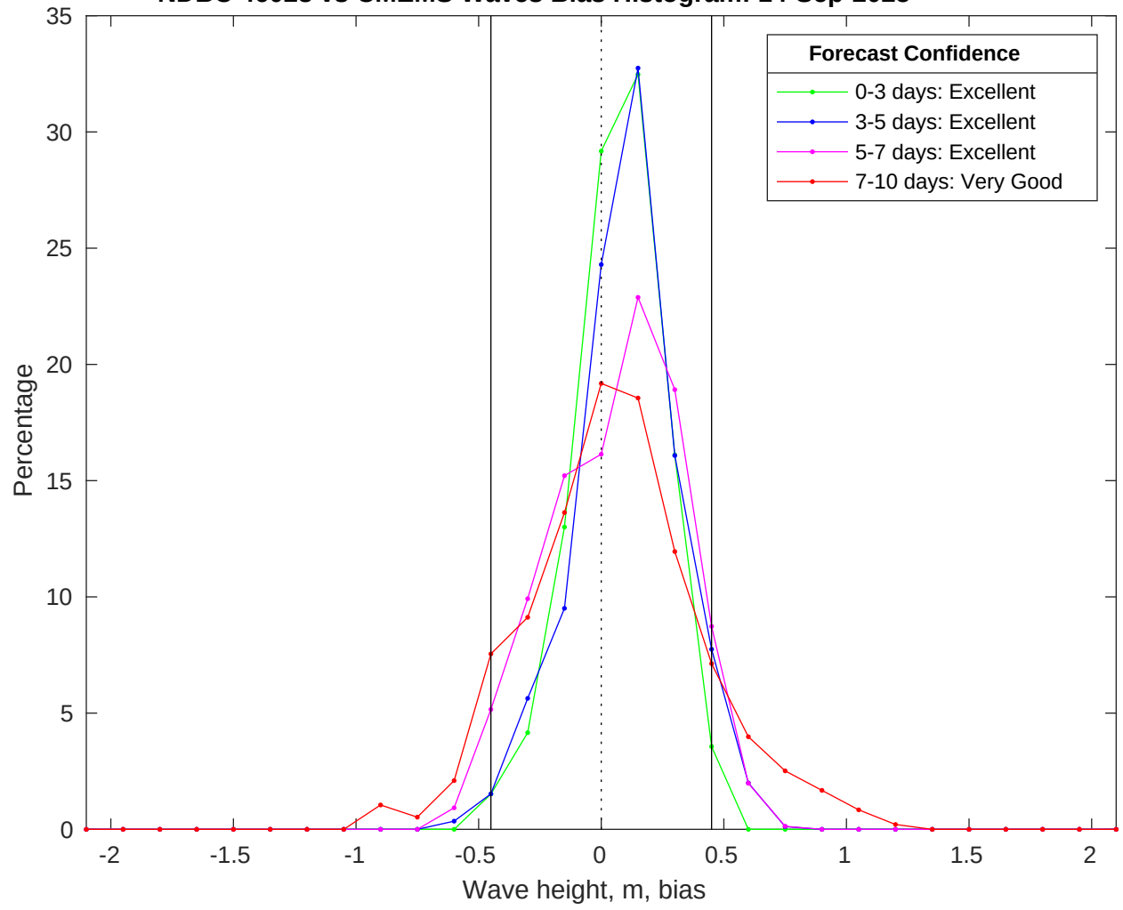
NDBC 46028 vs CMEMS Waves Bias Histogram: 14-Sep-2025
