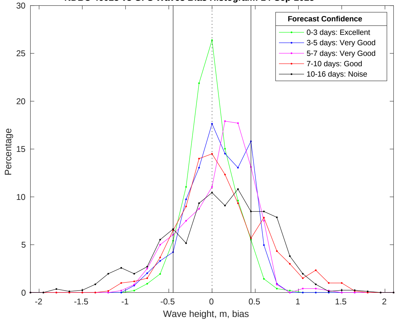
NDBC 46028 vs GFS Waves Bias Histogram: 14-Sep-2025
