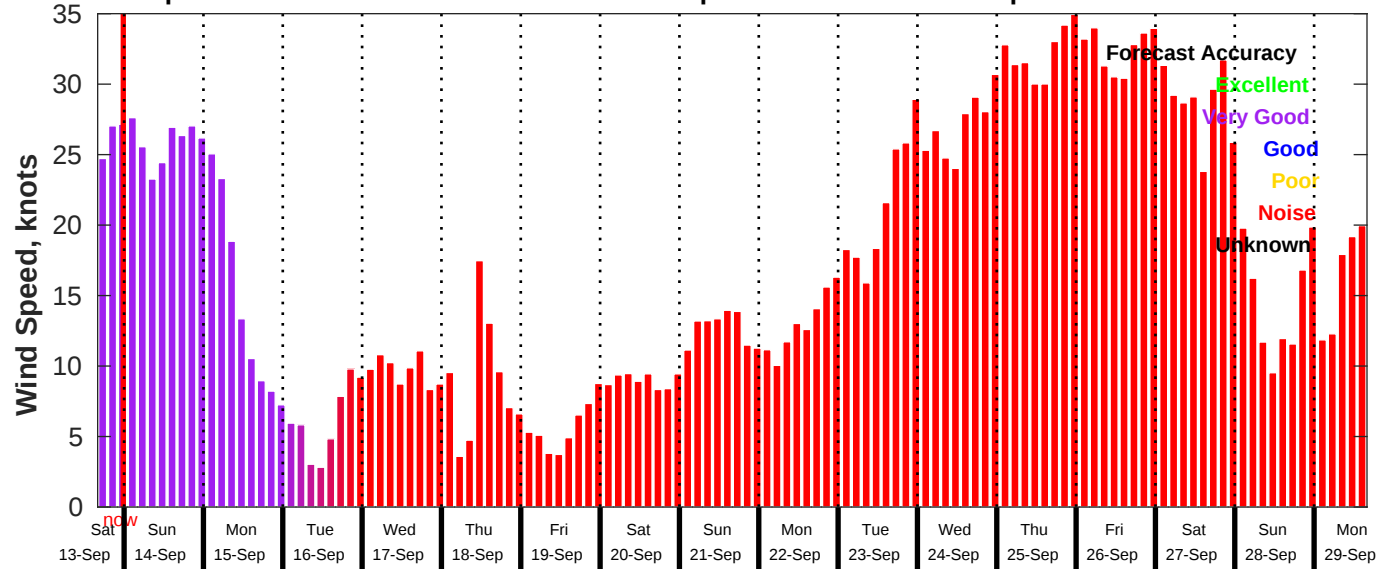
GFS Wind Speed Forecast for NDBC 46028 from 13-Sep-2025 16:00:00 to 29-Sep-2025 16:00:00
