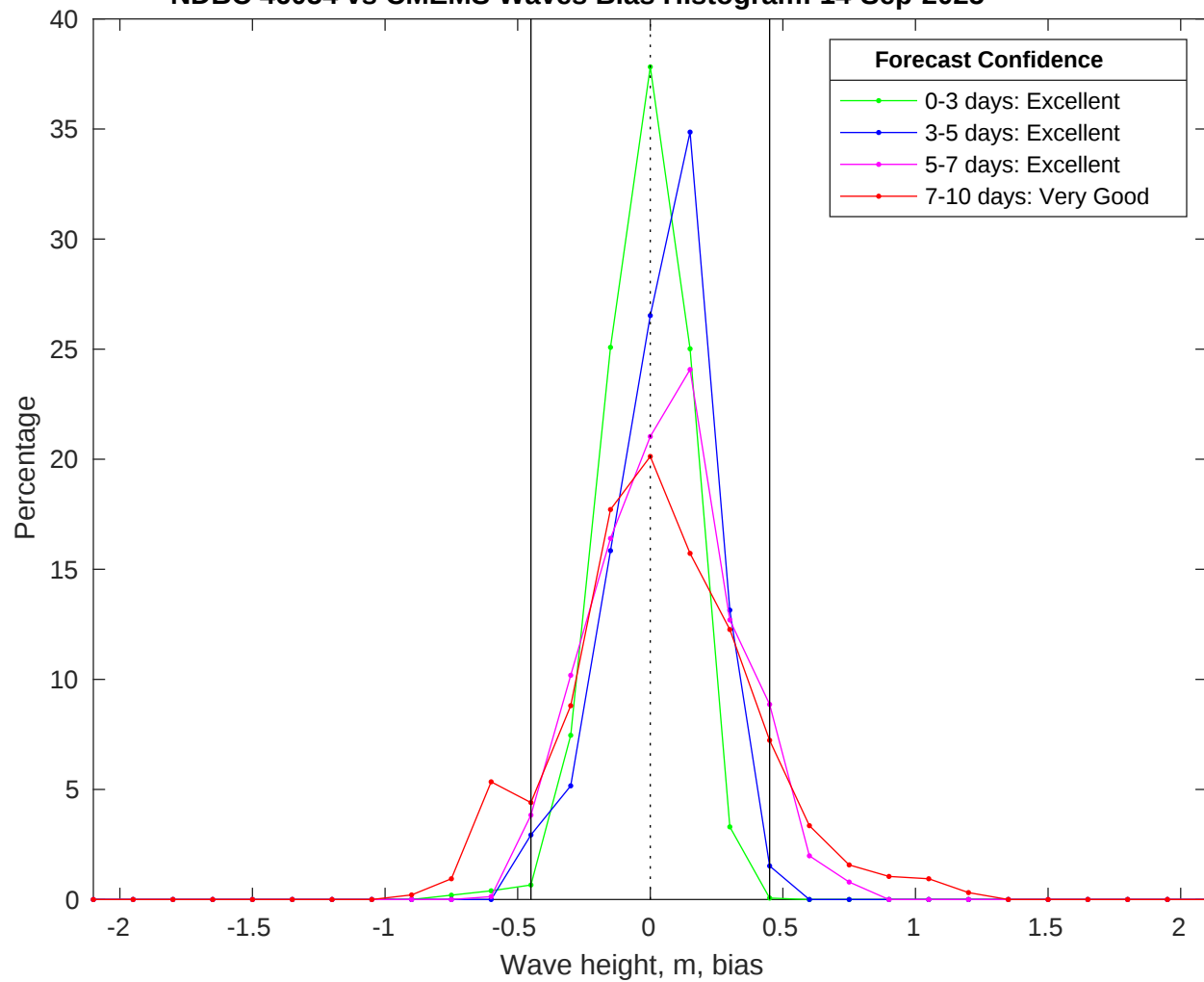
NDBC 46054 vs CMEMS Waves Bias Histogram: 14-Sep-2025
