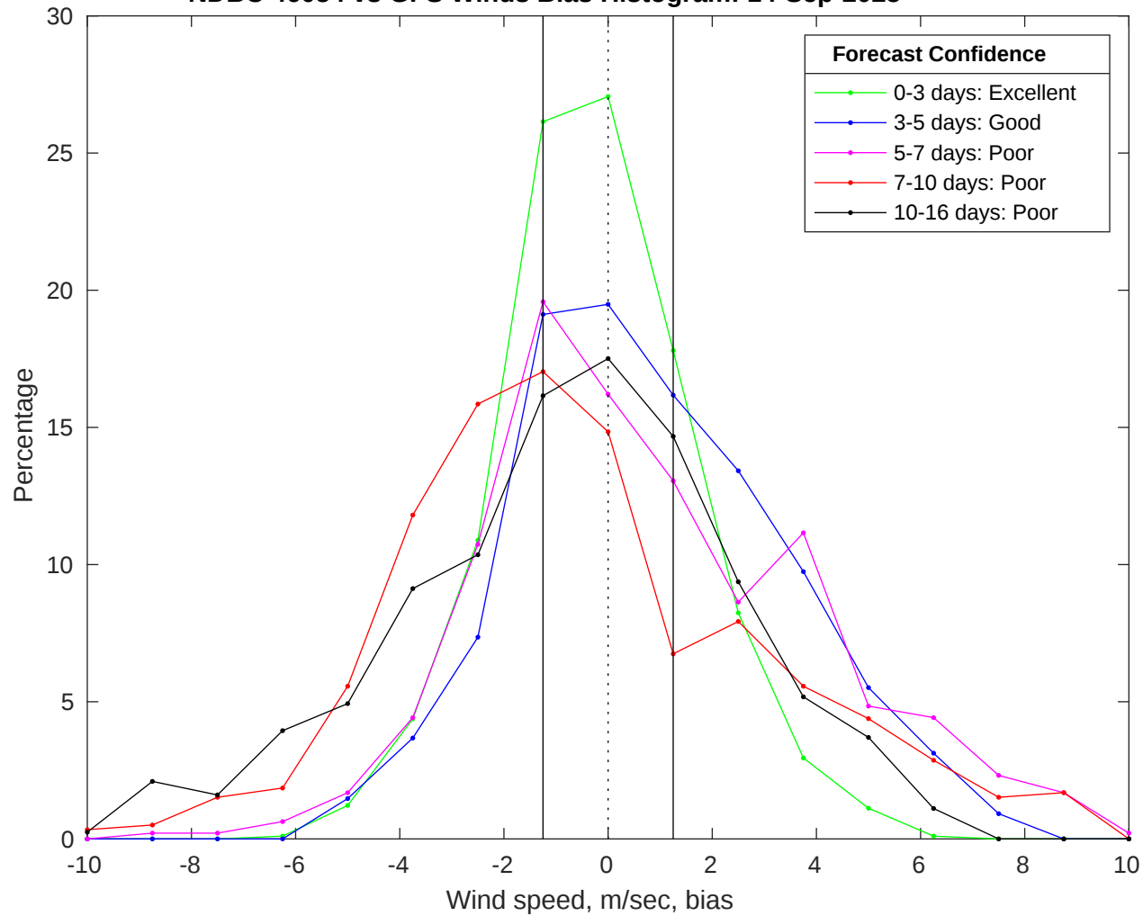
NDBC 46054 vs GFS Winds Bias Histogram: 14-Sep-2025
