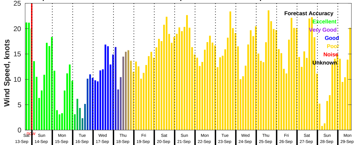
GFS Wind Speed Forecast for NDBC 46054 from 13-Sep-2025 16:00:00 to 29-Sep-2025 16:00:00
