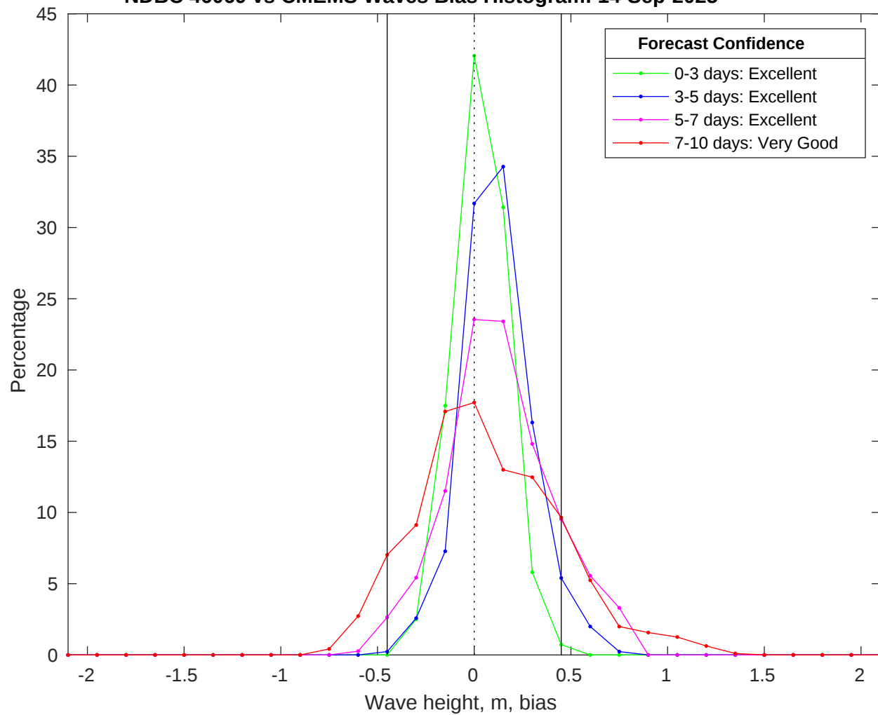
NDBC 46069 vs CMEMS Waves Bias Histogram: 14-Sep-2025
