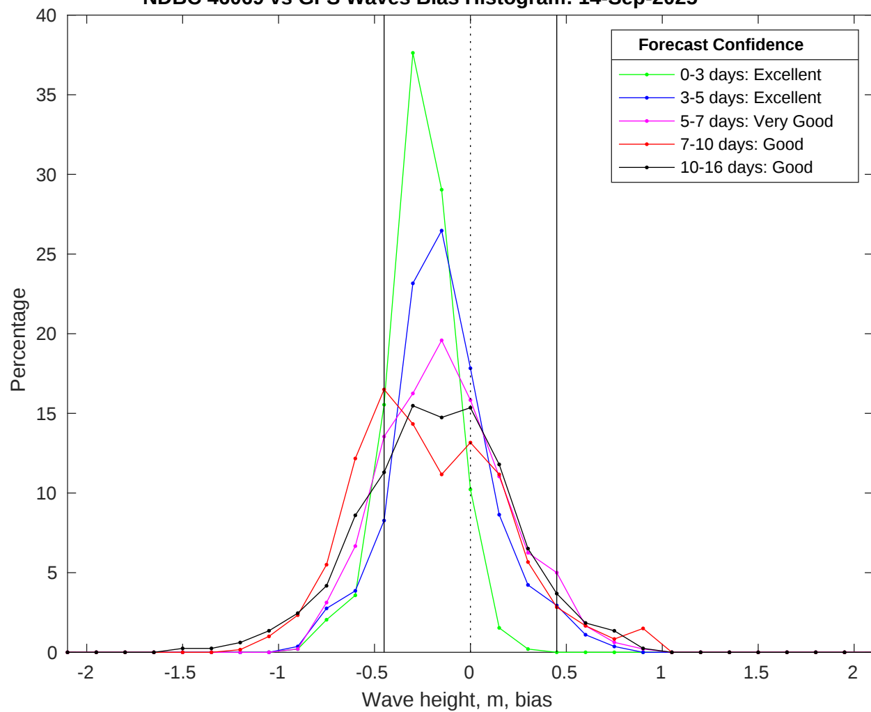
NDBC 46069 vs GFS Waves Bias Histogram: 14-Sep-2025
