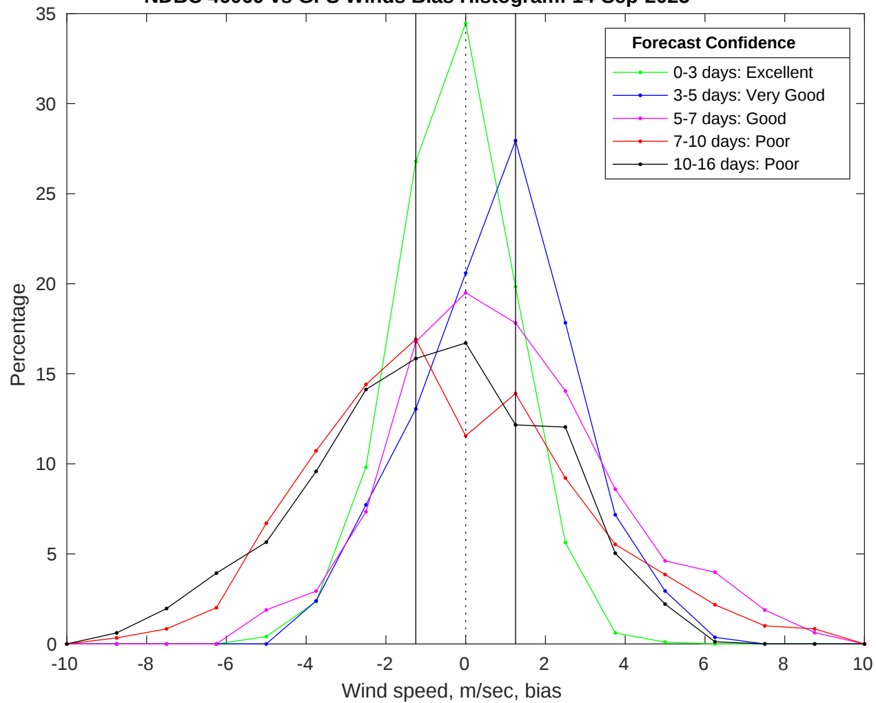
NDBC 46069 vs GFS Winds Bias Histogram: 14-Sep-2025
