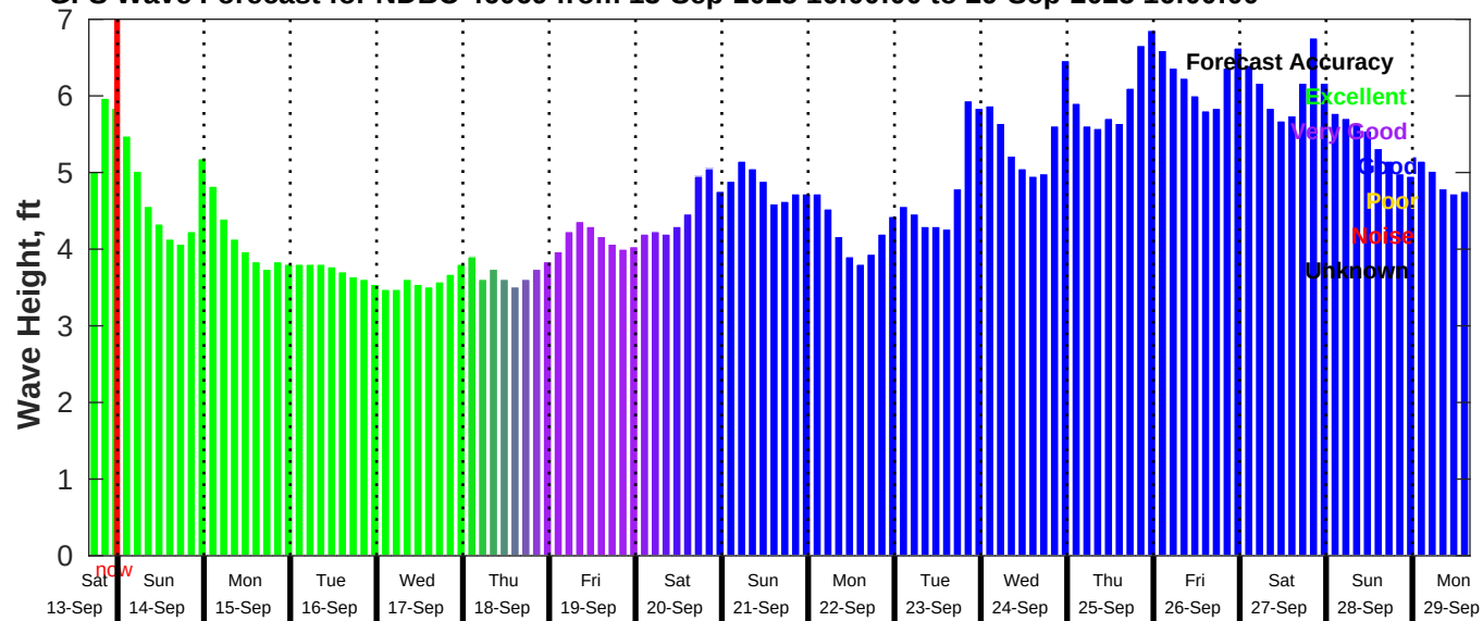
GFS Wave Forecast for NDBC 46069 from 13-Sep-2025 16:00:00 to 29-Sep-2025 16:00:00
