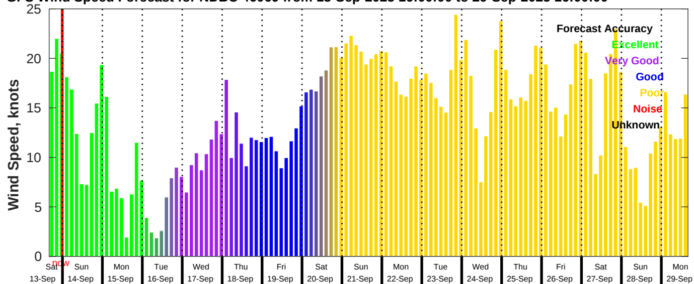
GFS Wind Speed Forecast for NDBC 46069 from 13-Sep-2025 16:00:00 to 29-Sep-2025 16:00:00
