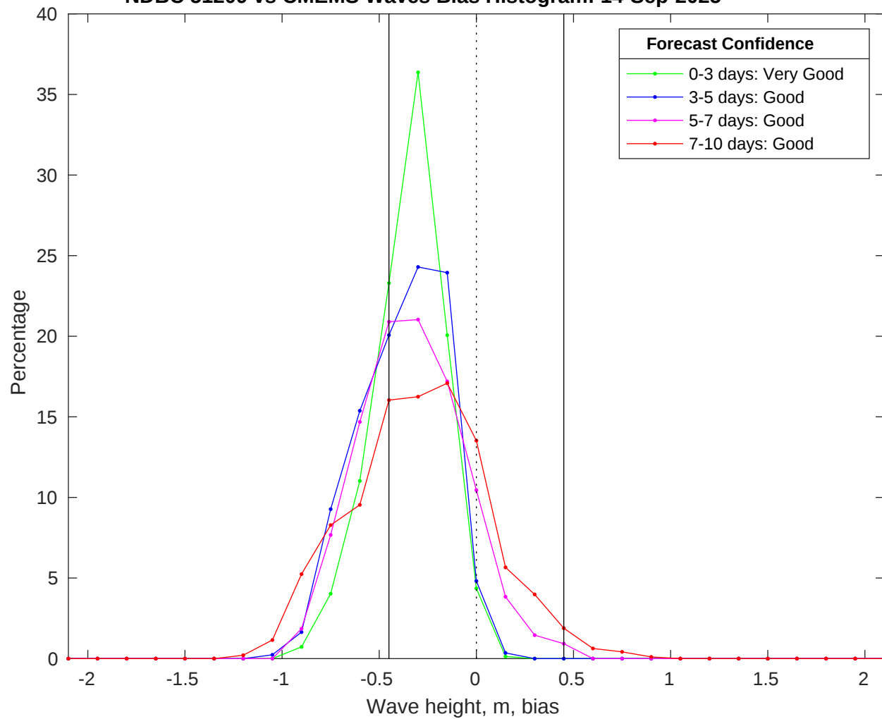
NDBC 51209 vs CMEMS Waves Bias Histogram: 14-Sep-2025
