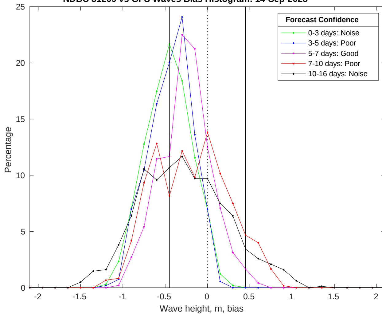
NDBC 51209 vs GFS Waves Bias Histogram: 14-Sep-2025
