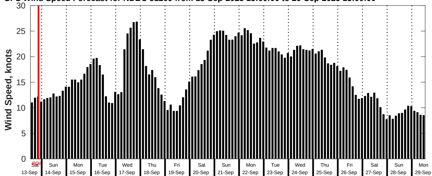
GFS Wind Speed Forecast for NDBC 51209 from 13-Sep-2025 13:00:00 to 29-Sep-2025 13:00:00
