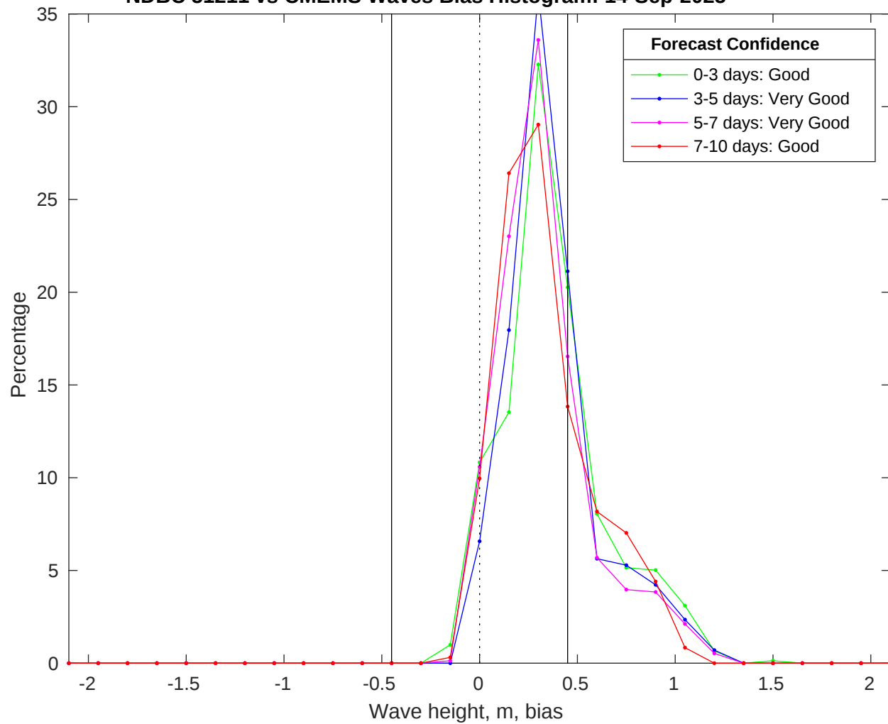
NDBC 51211 vs CMEMS Waves Bias Histogram: 14-Sep-2025
