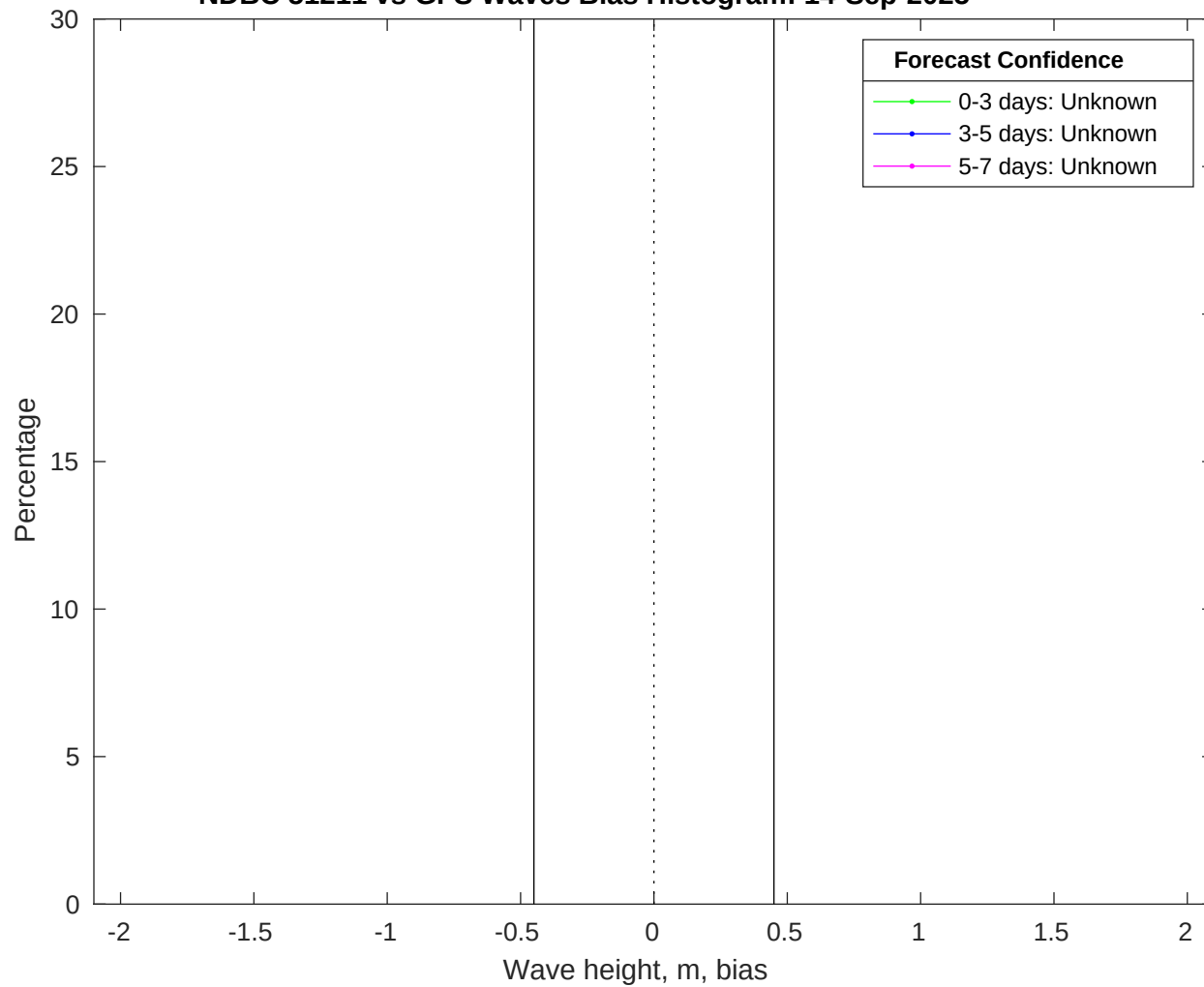
NDBC 51211 vs GFS Waves Bias Histogram: 14-Sep-2025
