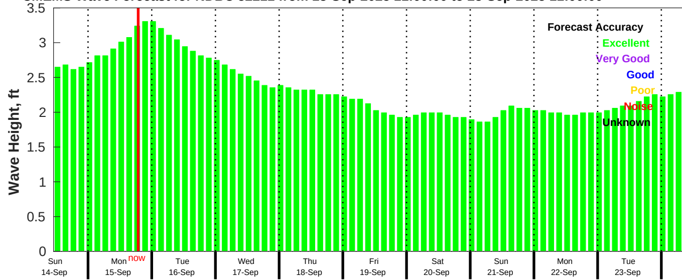
CMEMS Wave Forecast for NDBC 52211 from 13-Sep-2025 11:00:00 to 23-Sep-2025 11:00:00
