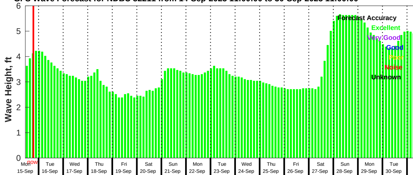
GFS Wave Forecast for NDBC 52211 from 14-Sep-2025 11:00:00 to 30-Sep-2025 11:00:00
