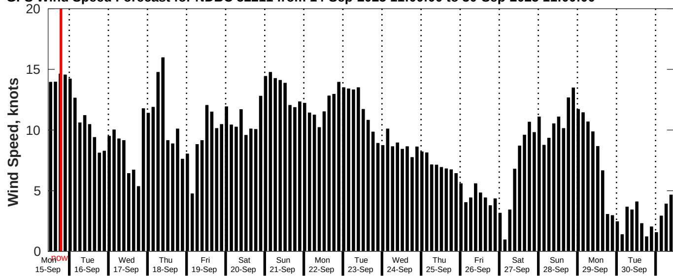
GFS Wind Speed Forecast for NDBC 52211 from 14-Sep-2025 11:00:00 to 30-Sep-2025 11:00:00
