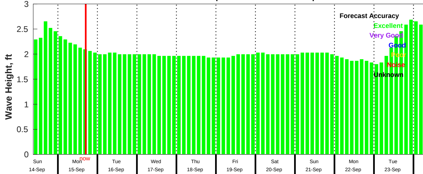
CMEMS Wave Forecast for NDBC 52212 from 13-Sep-2025 09:00:00 to 23-Sep-2025 09:00:00
