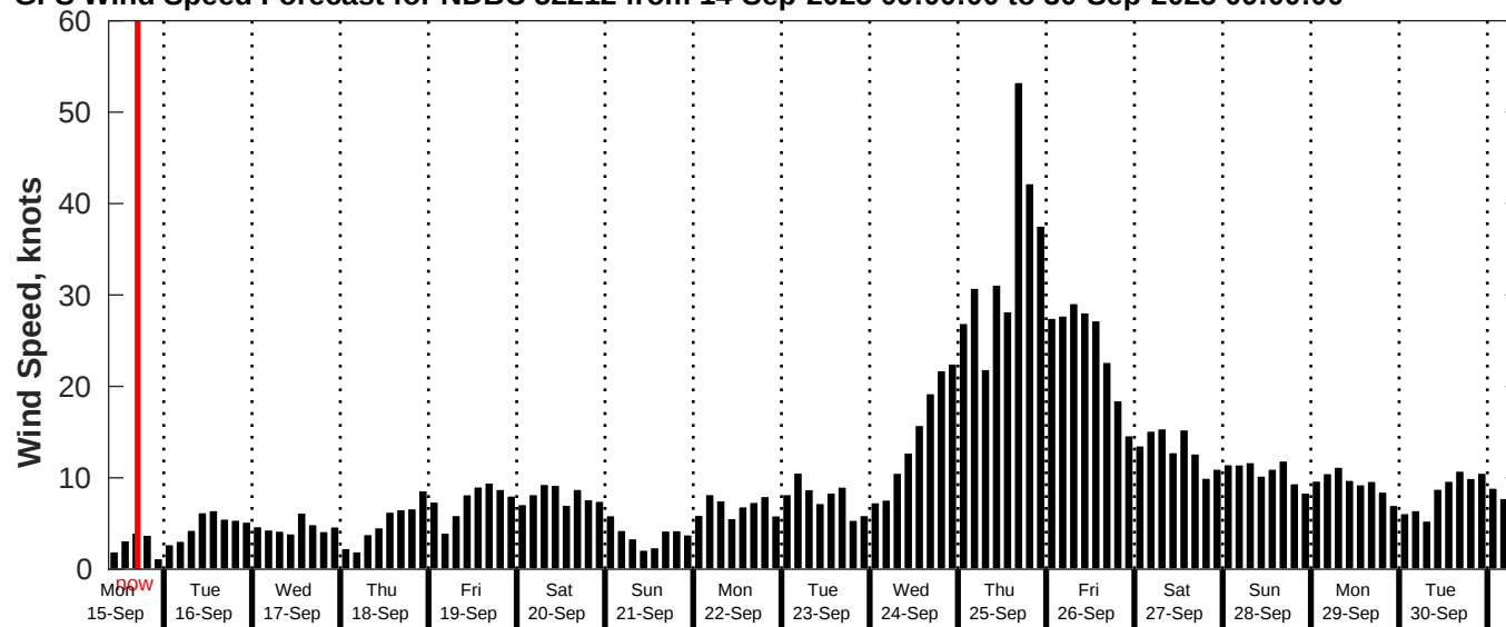
GFS Wind Speed Forecast for NDBC 52212 from 14-Sep-2025 09:00:00 to 30-Sep-2025 09:00:00
