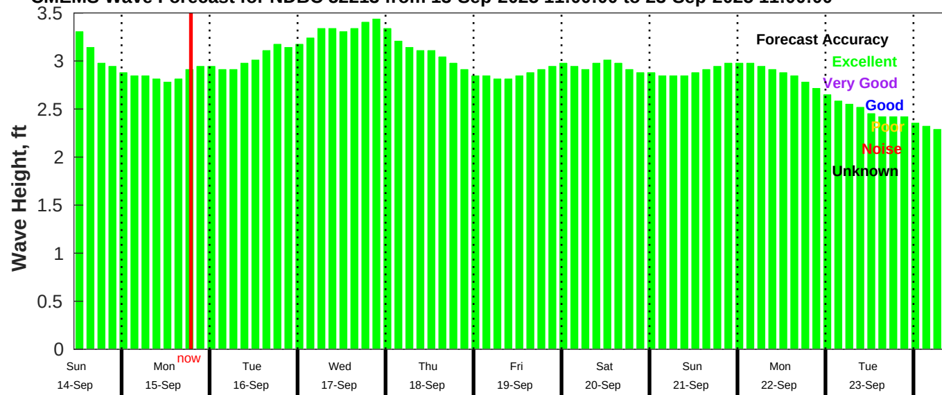
CMEMS Wave Forecast for NDBC 52213 from 13-Sep-2025 11:00:00 to 23-Sep-2025 11:00:00
