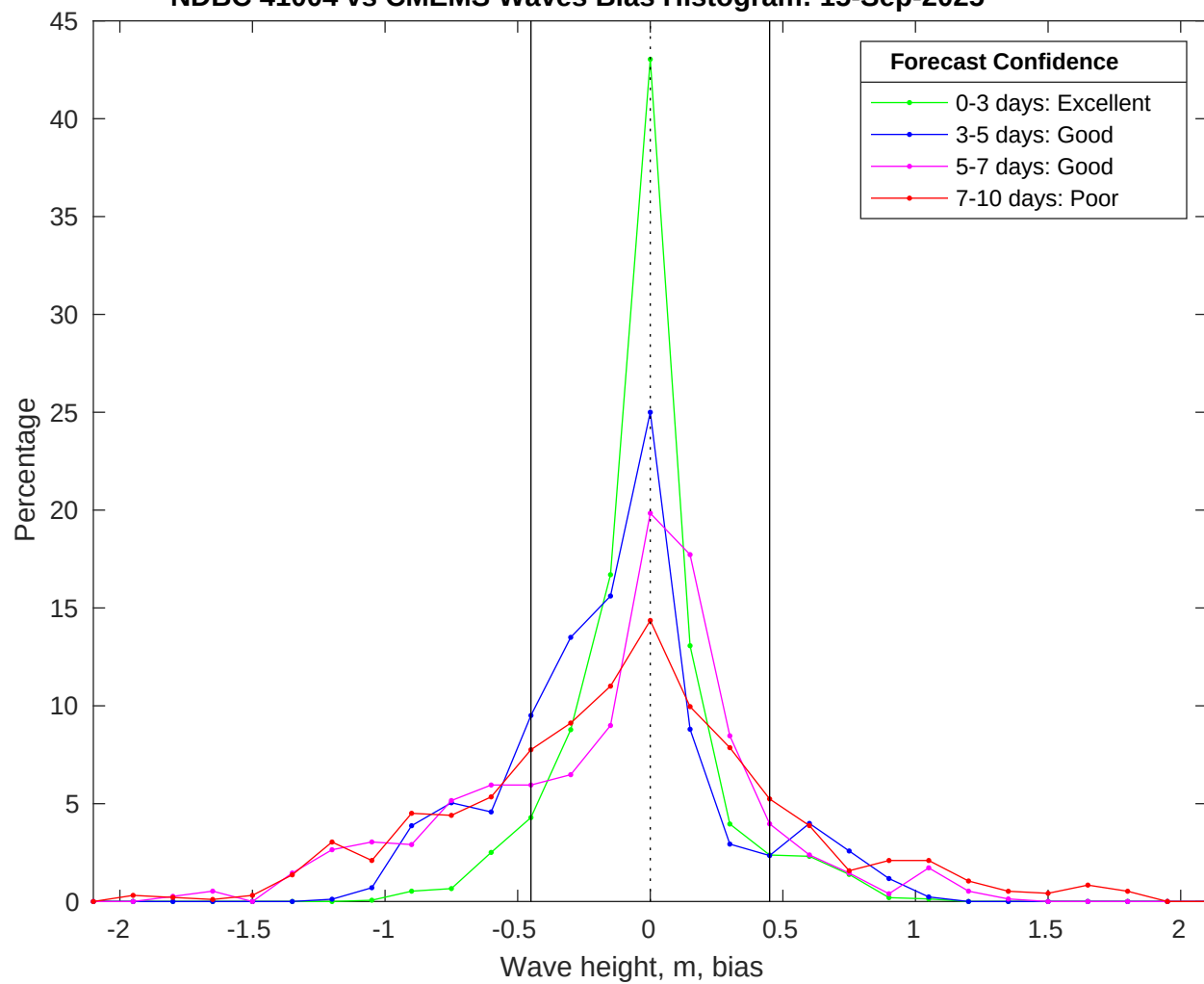
NDBC 41004 vs CMEMS Waves Bias Histogram: 15-Sep-2025
