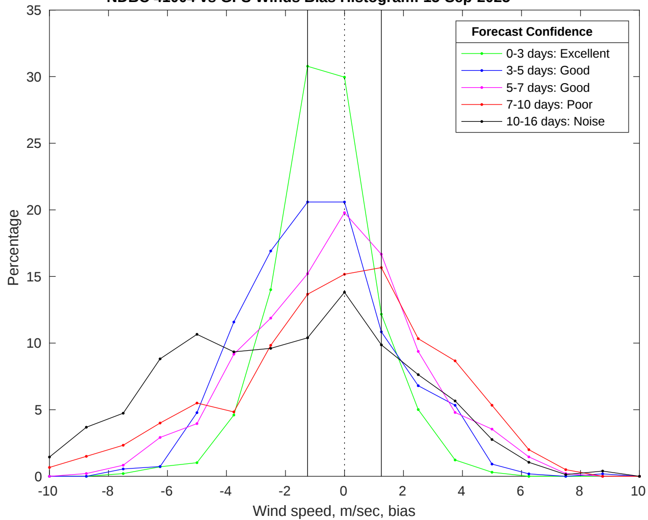
NDBC 41004 vs GFS Winds Bias Histogram: 15-Sep-2025
