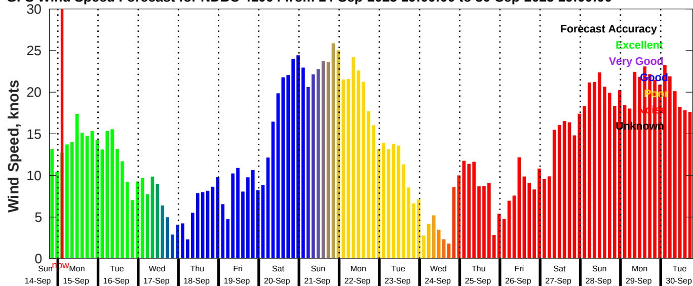
GFS Wind Speed Forecast for NDBC 41004 from 14-Sep-2025 19:00:00 to 30-Sep-2025 19:00:00
