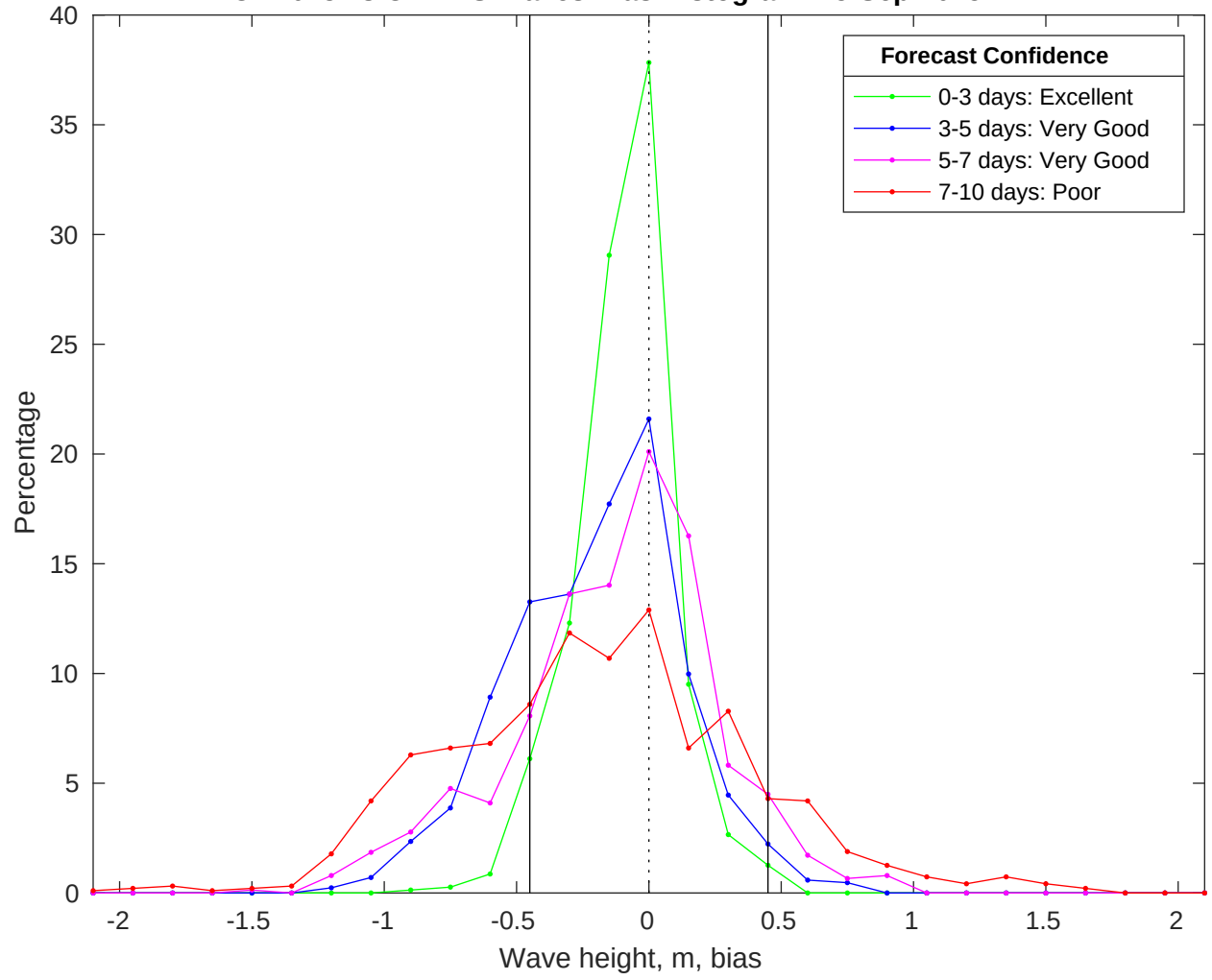
NDBC 41013 vs CMEMS Waves Bias Histogram: 15-Sep-2025
