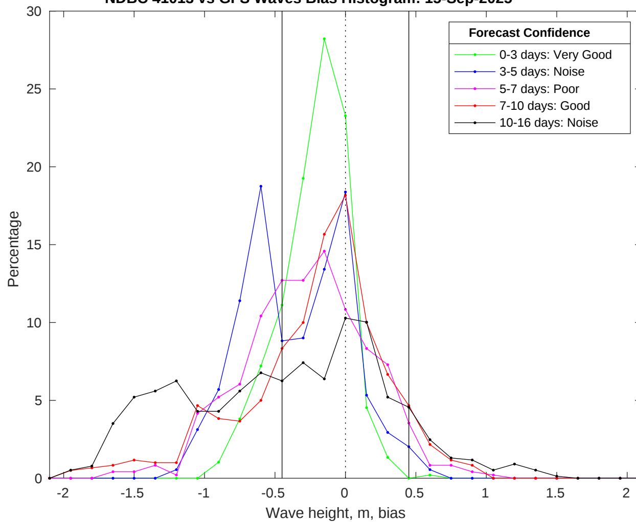
NDBC 41013 vs GFS Waves Bias Histogram: 15-Sep-2025
