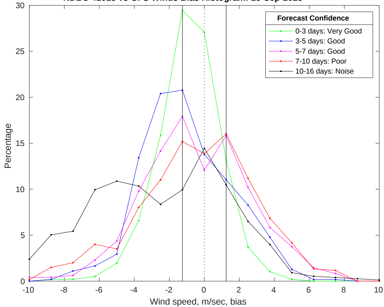
NDBC 41013 vs GFS Winds Bias Histogram: 15-Sep-2025
