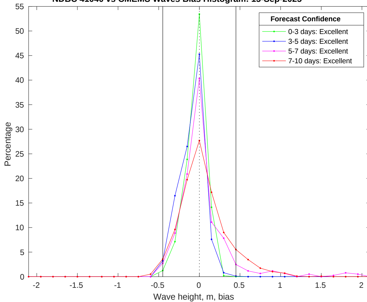
NDBC 41040 vs CMEMS Waves Bias Histogram: 15-Sep-2025
