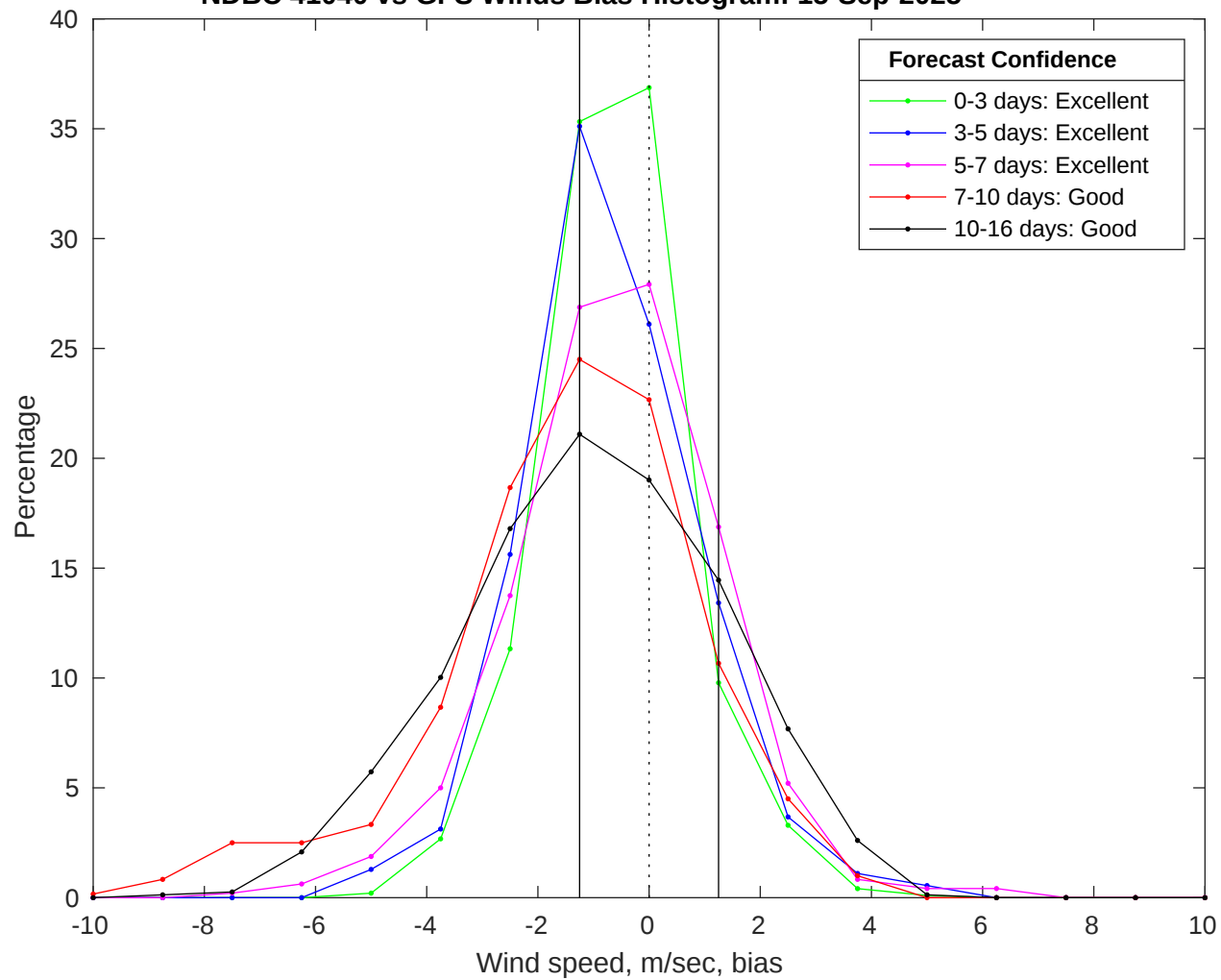
NDBC 41040 vs GFS Winds Bias Histogram: 15-Sep-2025
