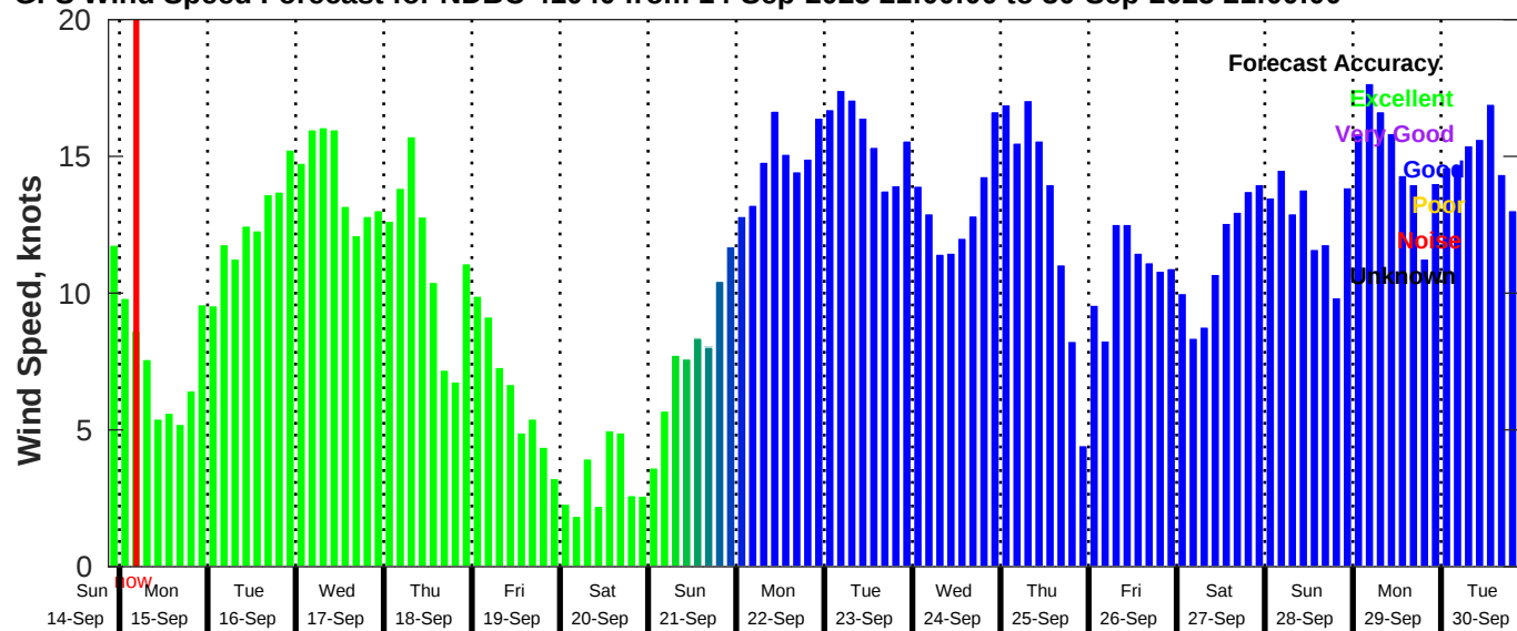
GFS Wind Speed Forecast for NDBC 41040 from 14-Sep-2025 21:00:00 to 30-Sep-2025 21:00:00
