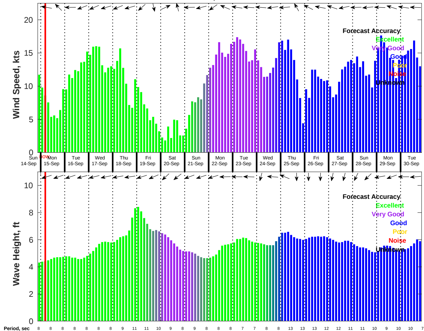
Wind & Wave Forecast for NDBC 41040 from 14-Sep-2025 21:00:00 to 30-Sep-2025 21:00:00
