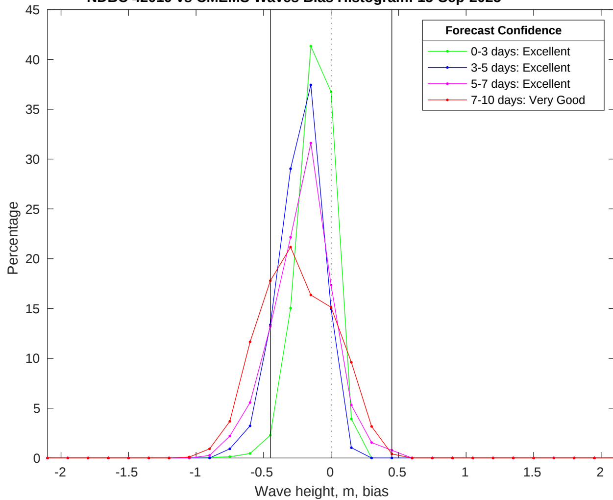
NDBC 42019 vs CMEMS Waves Bias Histogram: 15-Sep-2025
