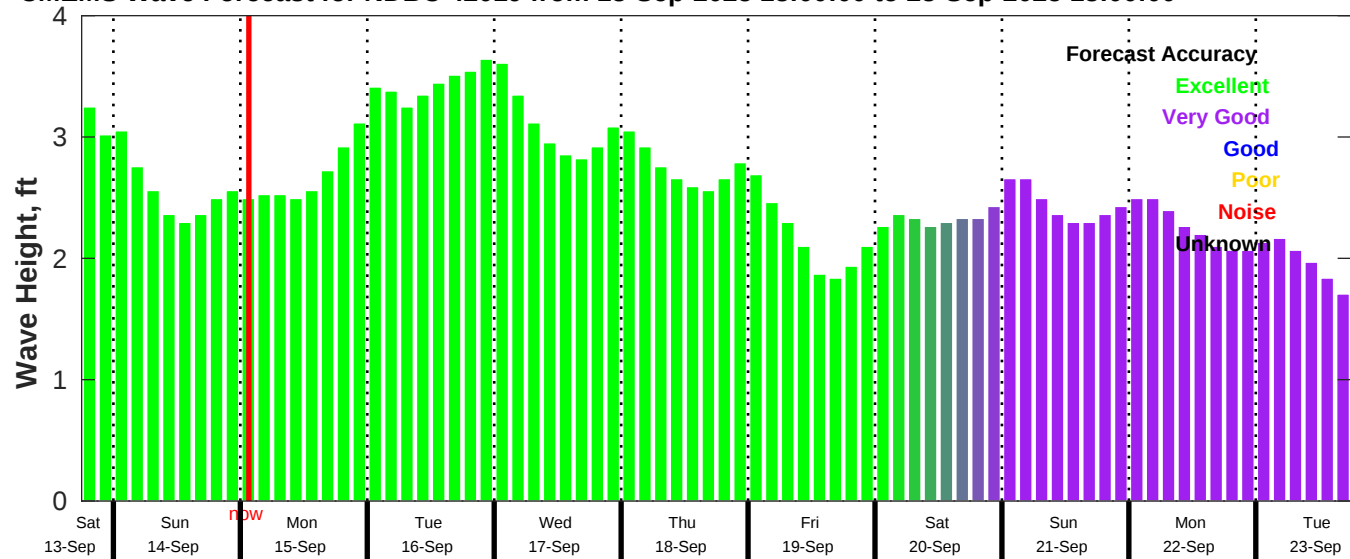
CMEMS Wave Forecast for NDBC 42019 from 13-Sep-2025 18:00:00 to 23-Sep-2025 18:00:00
