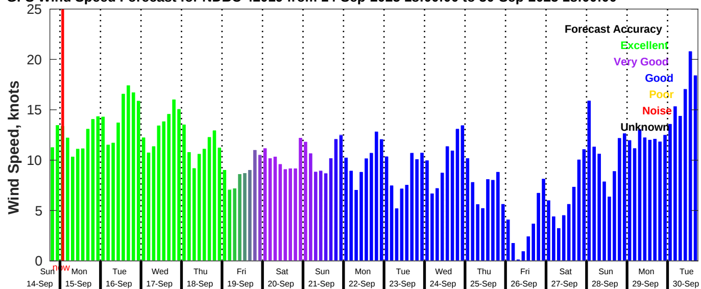
GFS Wind Speed Forecast for NDBC 42019 from 14-Sep-2025 18:00:00 to 30-Sep-2025 18:00:00
