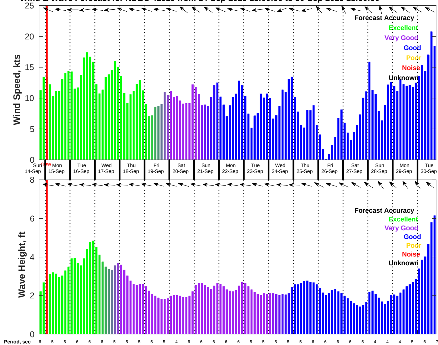
Wind & Wave Forecast for NDBC 42019 from 14-Sep-2025 18:00:00 to 30-Sep-2025 18:00:00
